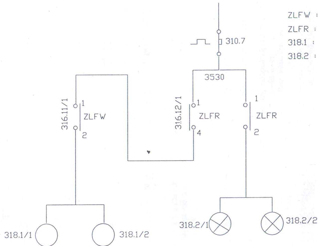
MODIFIED CIRCUIT DIAGRAM OF MARKER LIGHT.
